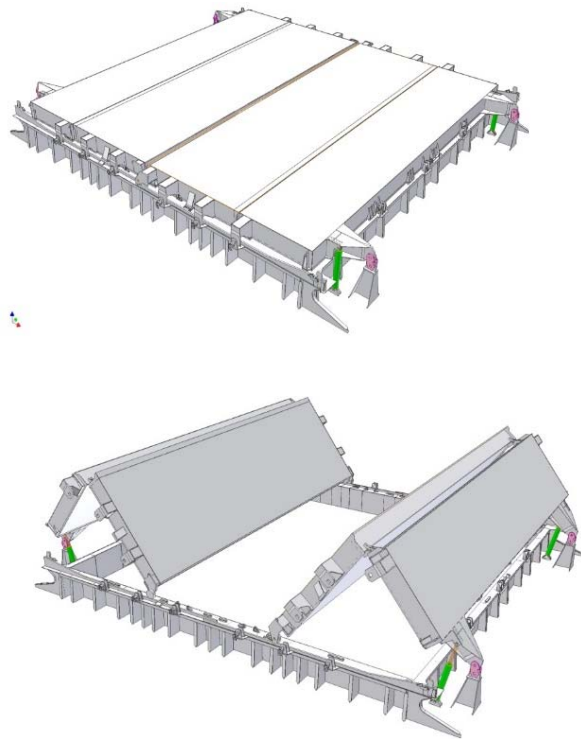
Single Folding Hatch Cover 单对折叠式舱盖
