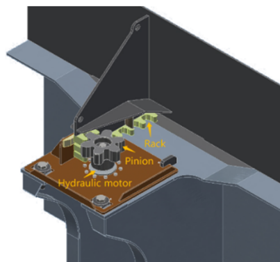
■ Rack and pinion drive 齿轮 齿条驱动
